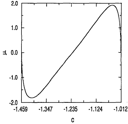
FIG. 1. Plot of \mu for c_L < c < c_R .
