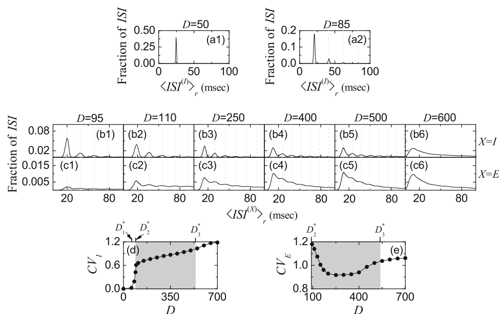
Fig. 5 Characterization of individual spiking behaviors in the absence of STDP. ISI histograms for D = \mathbf{a1} 50 and \mathbf{a2} 85 in the I-population. ISI histograms for various values of D in the I-population ( X = I ) ( \mathbf{b1} – \mathbf{b6} ) and the E-population ( X = E ) ( \mathbf{c1} – \mathbf{c6} ). Vertical dotted lines in \mathbf{a2} , \mathbf{b1} – \mathbf{b5} , and \mathbf{c1} – \mathbf{c5} represent multiples of the global period T_G^{(X)}
