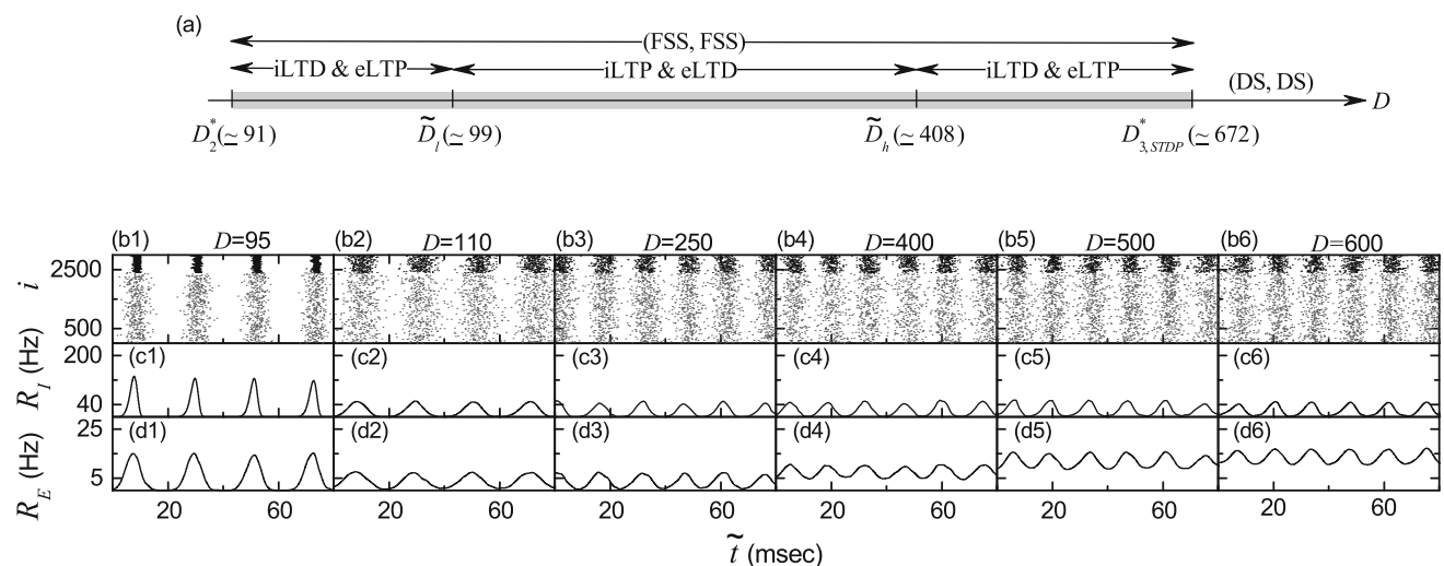
Fig. 8 Effects of interpopulation (I to E and E to I) STDPs on population states. a Bar diagram for the population states (I, E) in the I- and the E-populations. Raster plots of spikes in b1–b6 and instantaneous population spike rates R_I(t) in (c1–c6) and R_E(t) in
