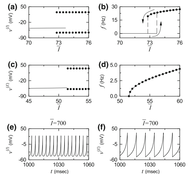
Fig. 2 Single Izhikevich fast spiking interneuron for D = 0 : a bifurcation diagram (i.e., plot of v^{(I)} versus the time-averaged constant \bar{I} of the external input I_{ext} ) and b plot of the mean firing rate f versus \bar{I} . Single Izhikevich regular spiking pyramidal cell for D = 0 : c bifurcation diagram (i.e., plot of v^{(E)} versus \bar{I} ) and d plot of f versus \bar{I} . In a , c , solid lines denote stable equilibrium points, and solid circles represent maximum and minimum values of the membrane potential v^{(X)} ( X = I or E ) for the spiking states. Time series of the membrane potential v^{(X)} of e the Izhikevich fast spiking interneuron and f the Izhikevich regular spiking pyramidal cell for \bar{I} = 700
